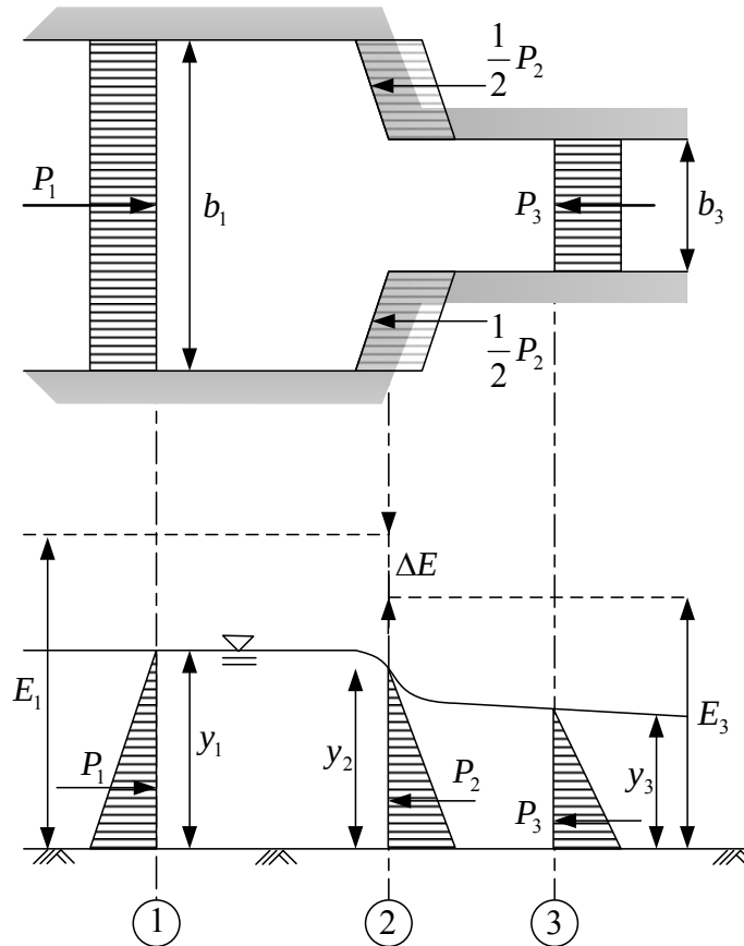
Figure 2-2-1 Contraction effect of the culvert
