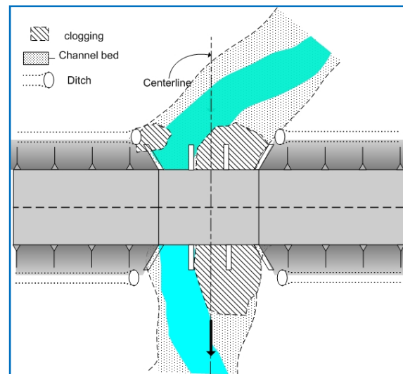
Culvert site sketch
