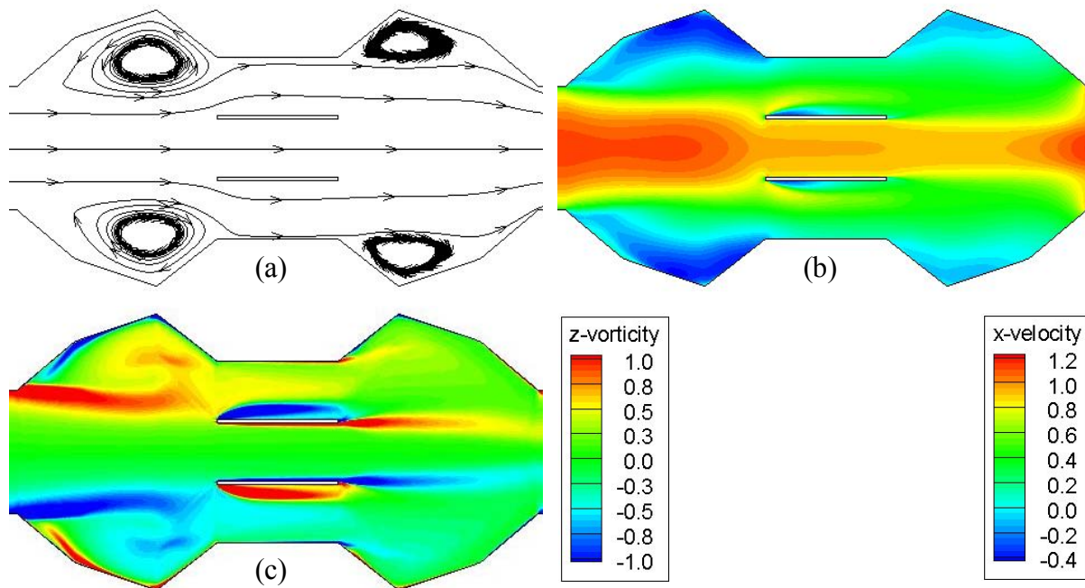
Figure 4-4-2 Near-surface flow field in flow Case B obtained with numerical simulations:
