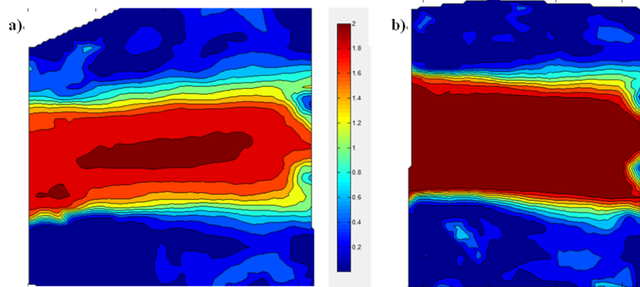
Figure 5-3-2 Velocity contours in the 1:5 model: a) reference condition, b) FA design model
