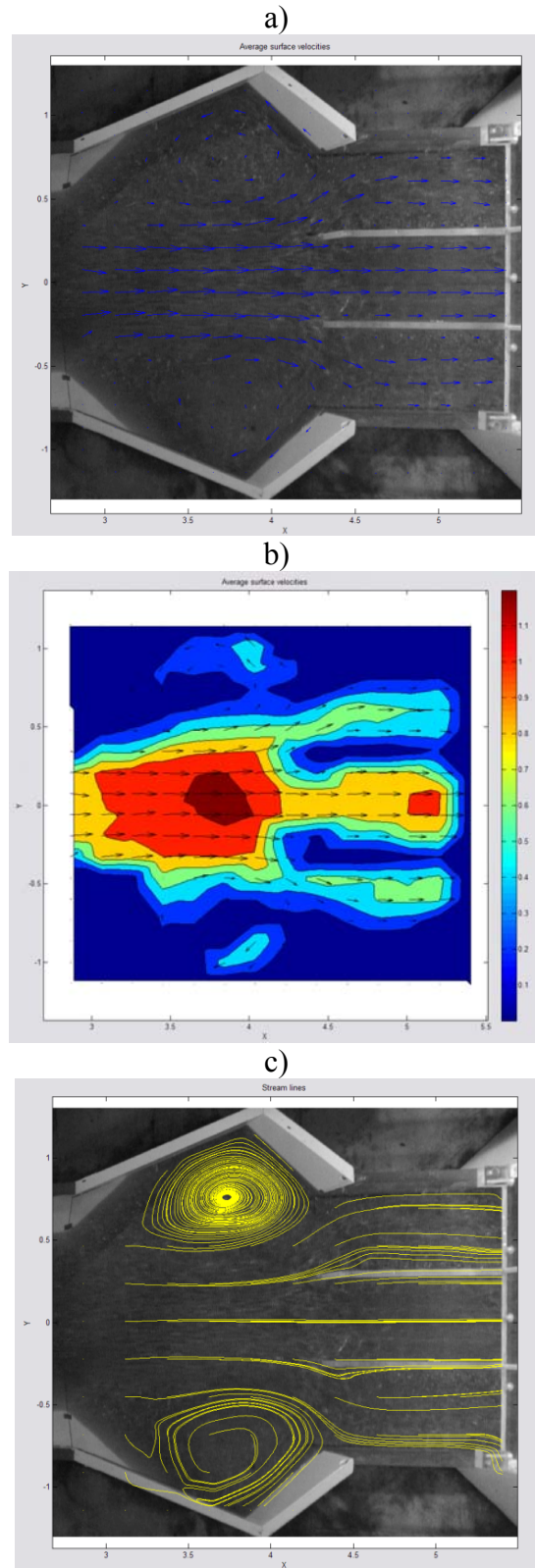
Figure 4-2-12 Surface flow field for case B ( HW/D=0.5 ): (a) Velocity vectors, (b) Velocity vectors and velocity magnitude contour, (c) Streamlines
