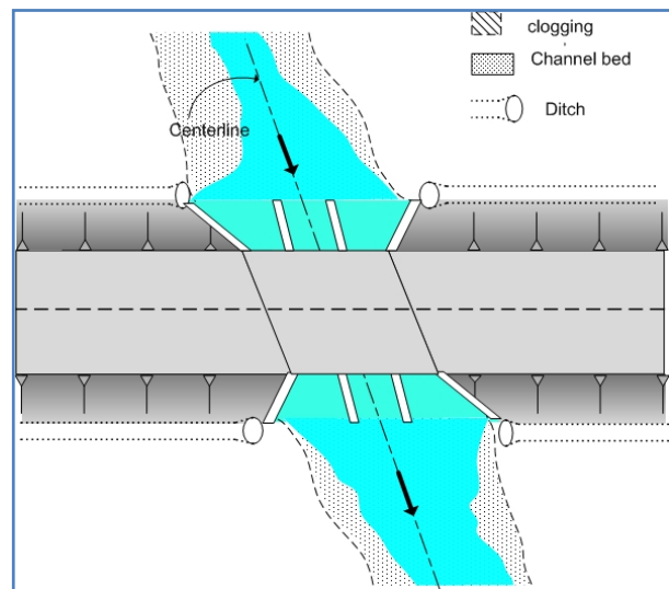
Culvert site sketch
