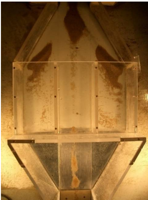
Figure 4-3-1 Sedimentation pattern compare to the baseline test result
