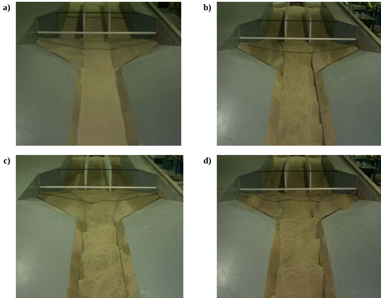
Figure 5-4-2 Sediment deposition patterns for the culvert fitted with fillets FA: a) Initial condition, b) flow Case A, c) flow Case B, d) flow Case C
