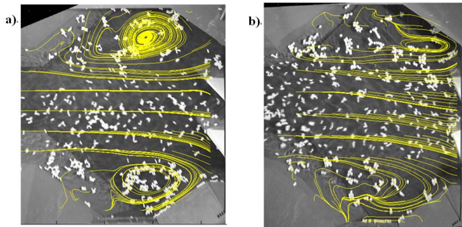
Figure 5-3-1 Streamlines in the 1:5 model: a) reference condition, b) FA design model
