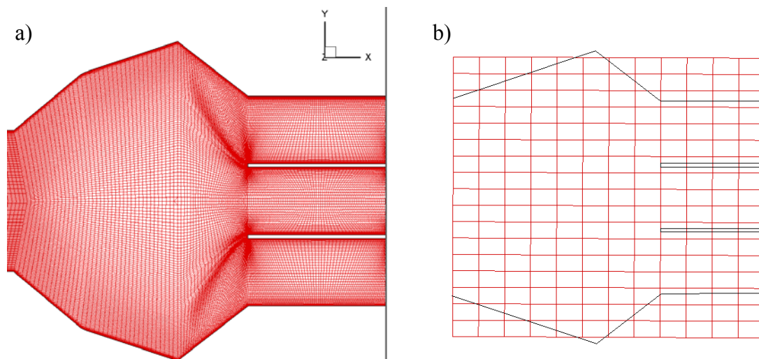
Figure 4-4-7 The mesh resolution: (a) the numerical model mesh, (b) the LSPIV analysis mesh
