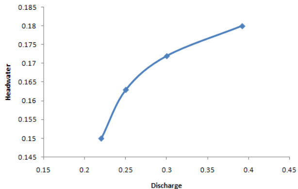
Figure 4-2-4. Trial flow conditions of the experiment
