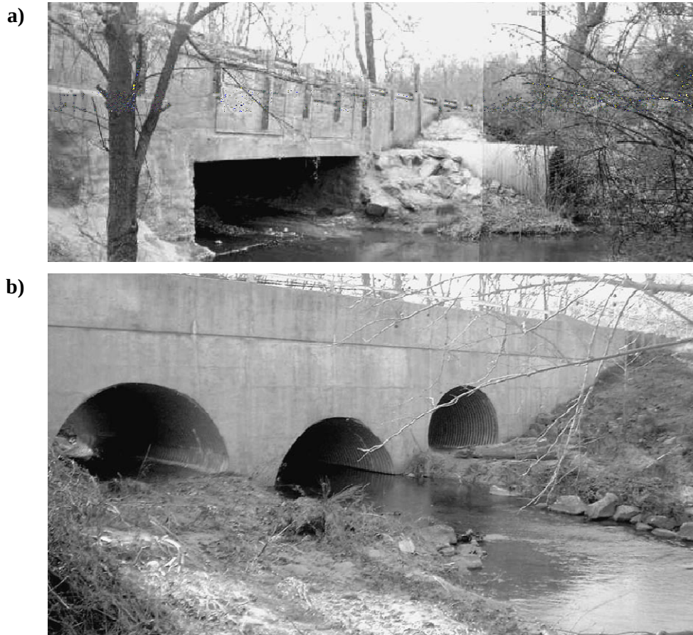
Figure 2-5-1: Culvert retrofitting using uneven inverts: a) pre-construction condition in 1992, b) post-construction in 2000
