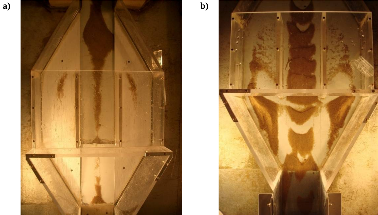
Figure 4-3-2 Sedimentation pattern compare to the baseline test result
