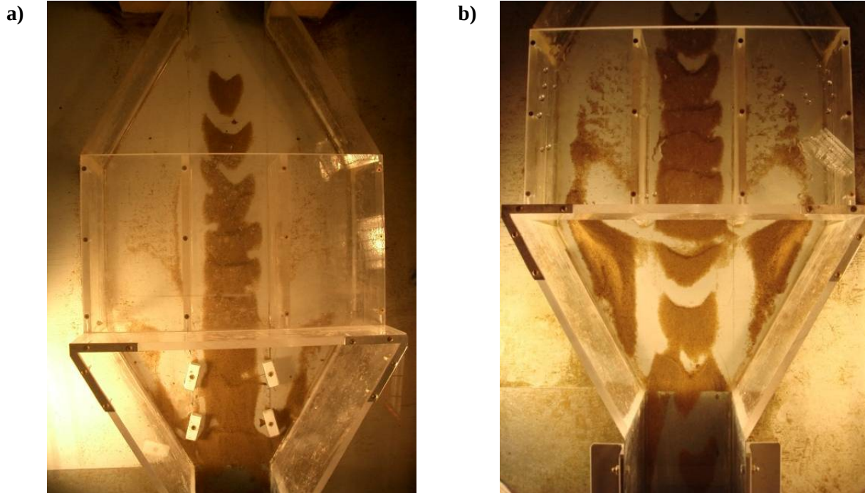
Figure 4-3-5 Sedimentation pattern compare to the baseline test result
