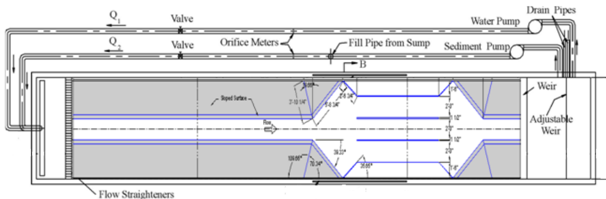
Figure 5-1-1. Schematic View of the physical model
