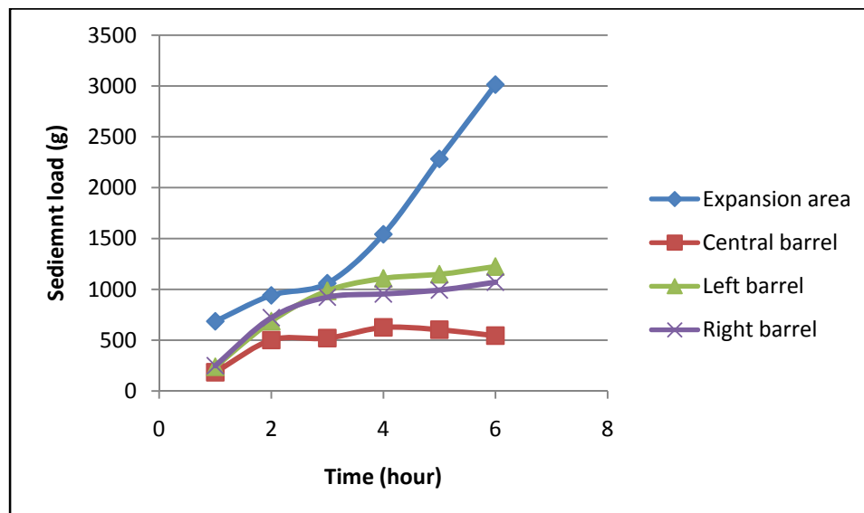
Figure 4-2-14 Rate of sediment accumulation in the culvert area for flow Case B
