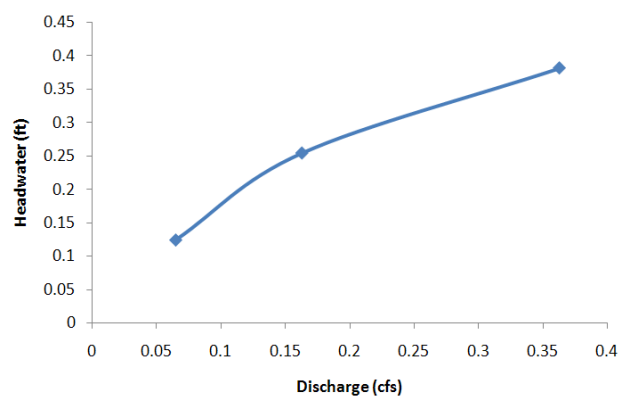
Figure 4-2-11 Flow condition in baseline test 3
