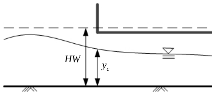
Figure 2-3-3 Culvert entrance acts like a weir
