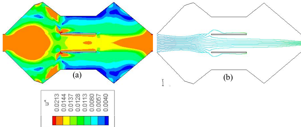
Figure 4-4-10 Simulated sediment transport characteristics for flow case B over fillets FA set in the expansion: (a) shear velocity, (b) sediment paths
