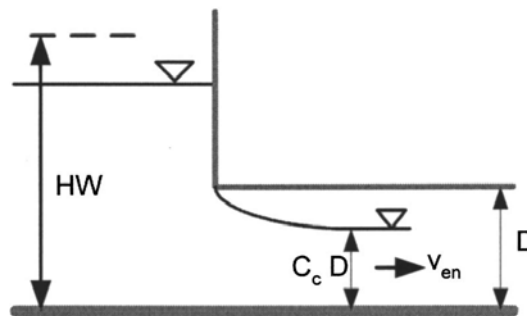
Figure 2-3-4 Culvert entrance acting as a submerged sluice gate (Charbeneau, 2006)
