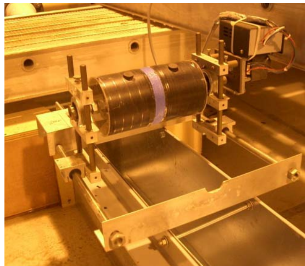
Figure 4-2-3 Sediment feeder
