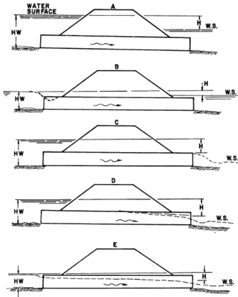
Figure 2-3-5 Types of outlet control (Normann, 1985)
