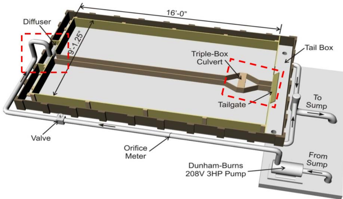
Figure 4-2-1 Overview of the flume
