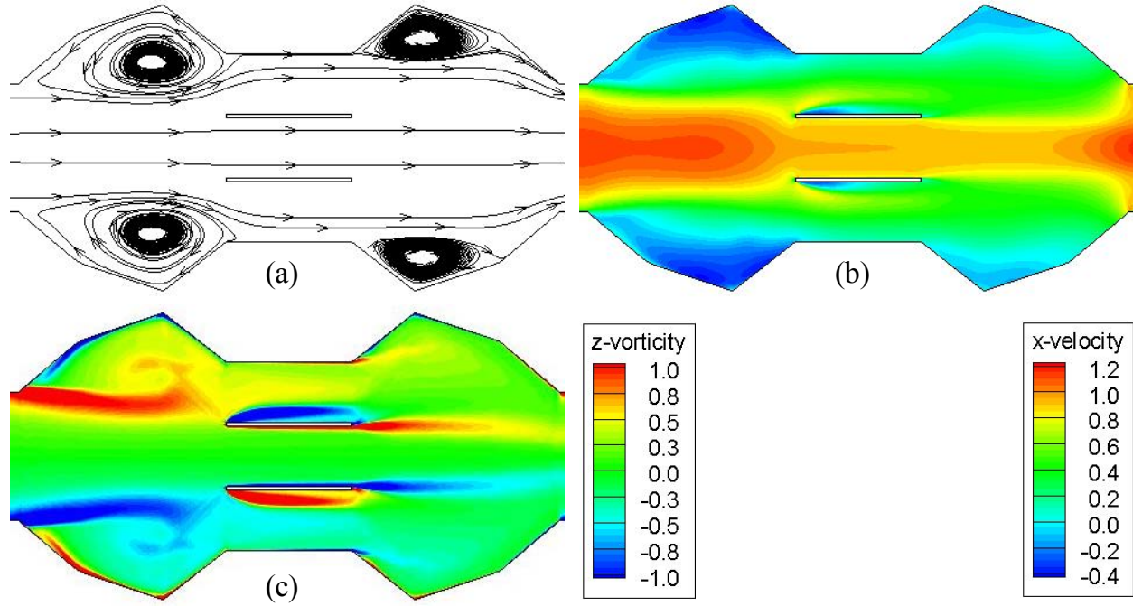
Figure 4-4-9 Simulated near-surface flow field for flow case B over the fillets FA set in the expansion: (a) streamlines, (b) streamwise velocity, (c) out of plane vorticity
