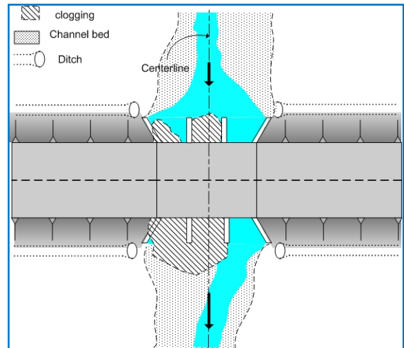
Culvert site sketch
