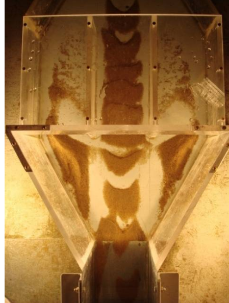
Figure 4-3-3 Sedimentation pattern compare to the baseline test result
