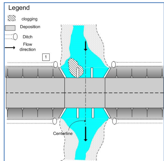
Culvert Sketch
