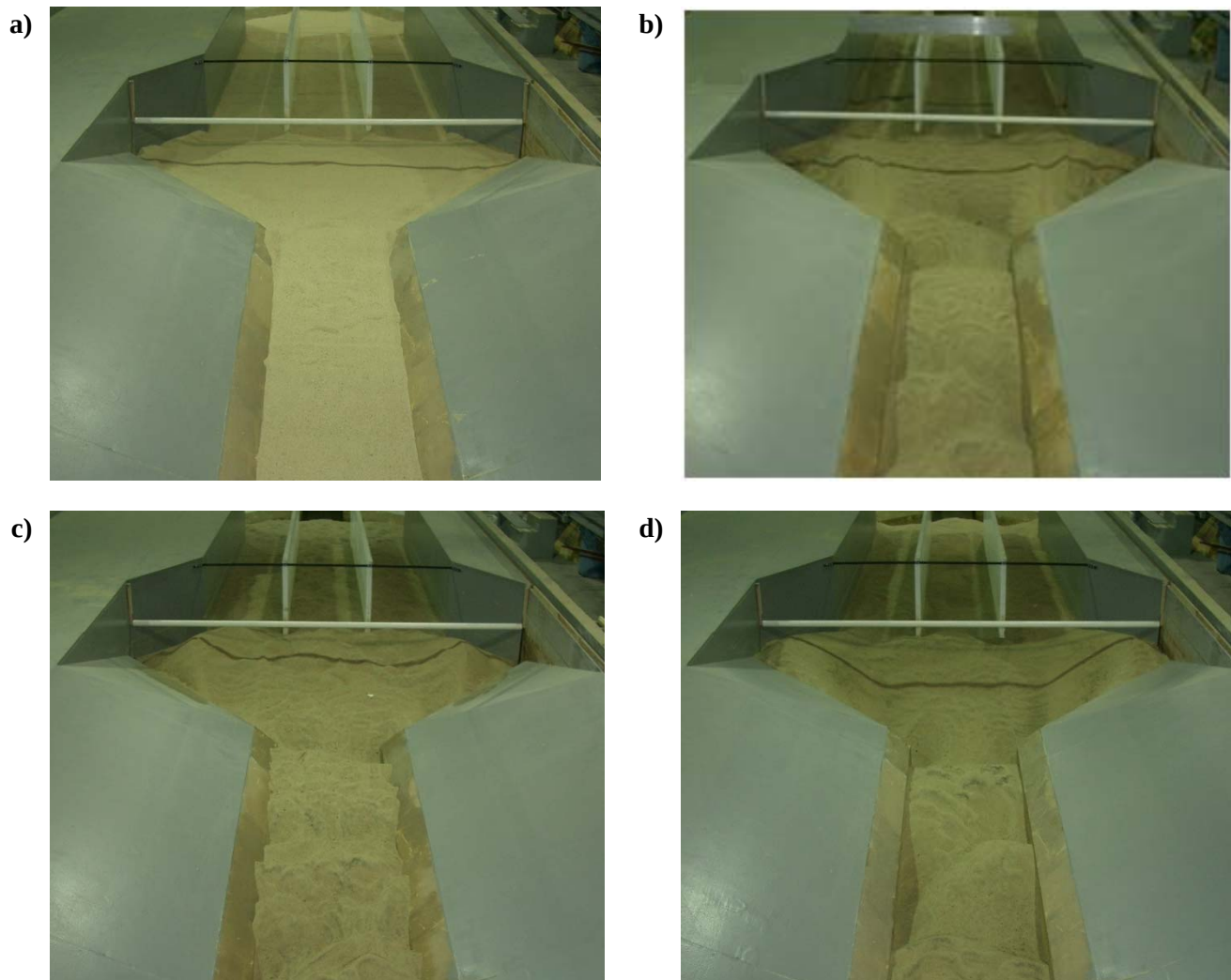
Figure 5-2-1 Sediment deposition patterns: a) Initial condition, b) Case A, c) Case B, d) Case C
