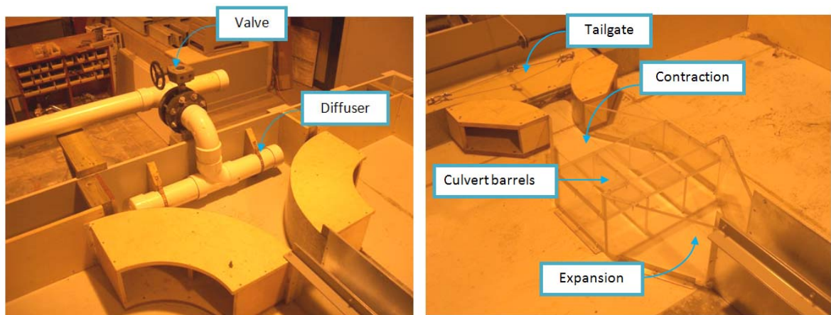
Figure 4-2-2 Layout of the culvert model
