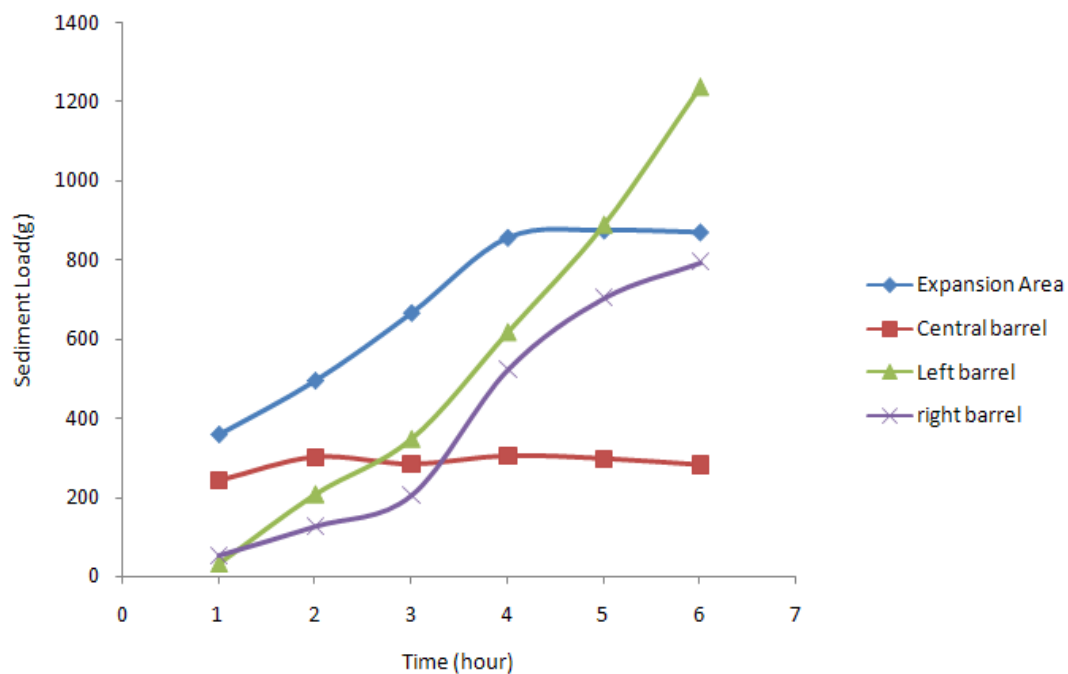
Figure 4-2-8 Rate of sediment accumulation in the expansion and three barrels
