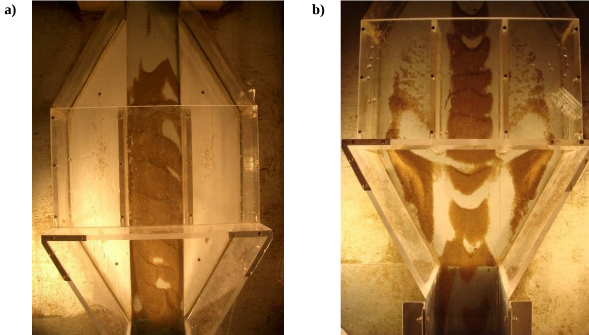
Figure 4-3-4 Sedimentation pattern compare to the baseline test result
