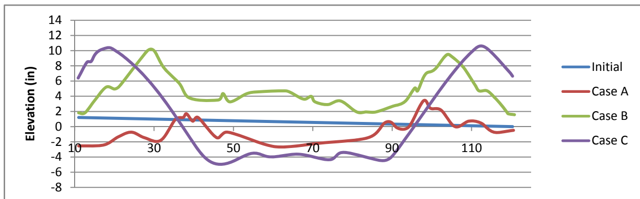
Figure 5-2-2 Elevation of sediment deposition at the cross-section under different flow conditions
