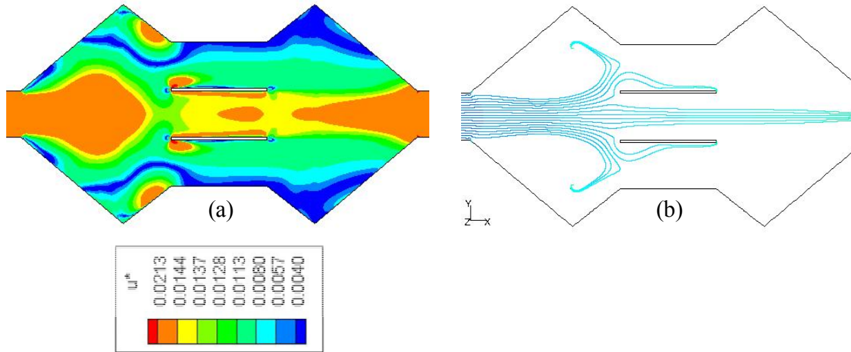
Figure 4-4-3 Sediment transport characteristics in flow Case B obtained from numerical simulations : (a) shear velocity, (b) sediment paths
