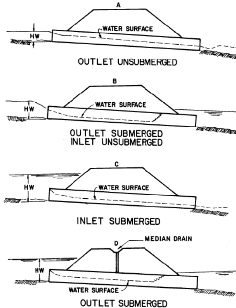
Figure 2-3-2 Types of inlet control, (Normann, 1985)
