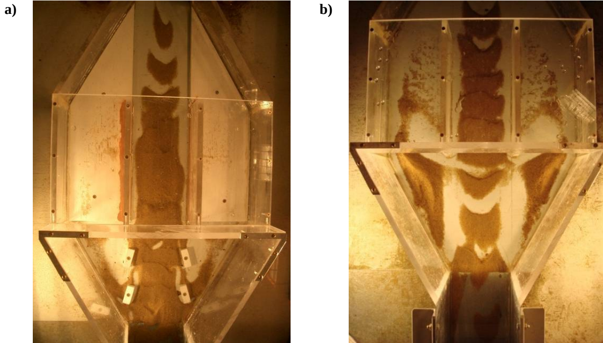
Figure 4-3-6 Sedimentation pattern compare to the baseline test result
