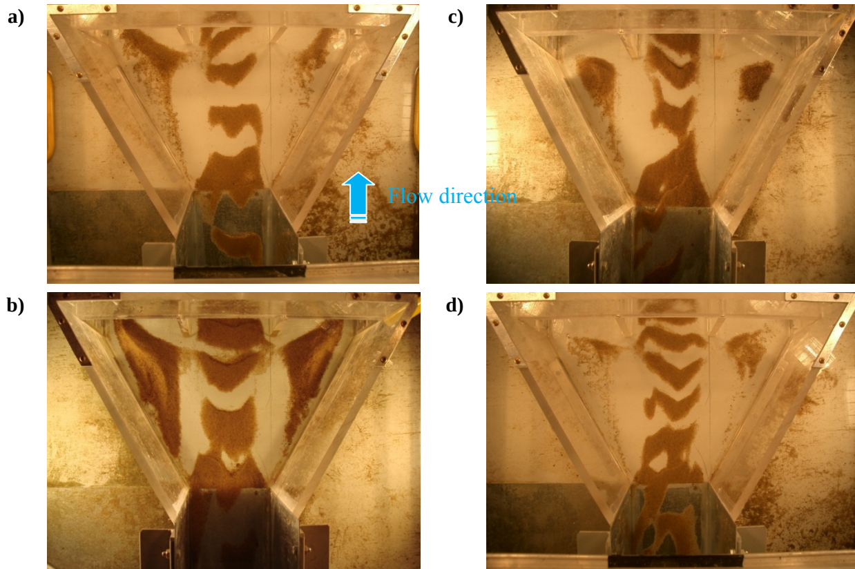
Figure 4-2-5 Sediment accumulation upstream of the culvert inlet
