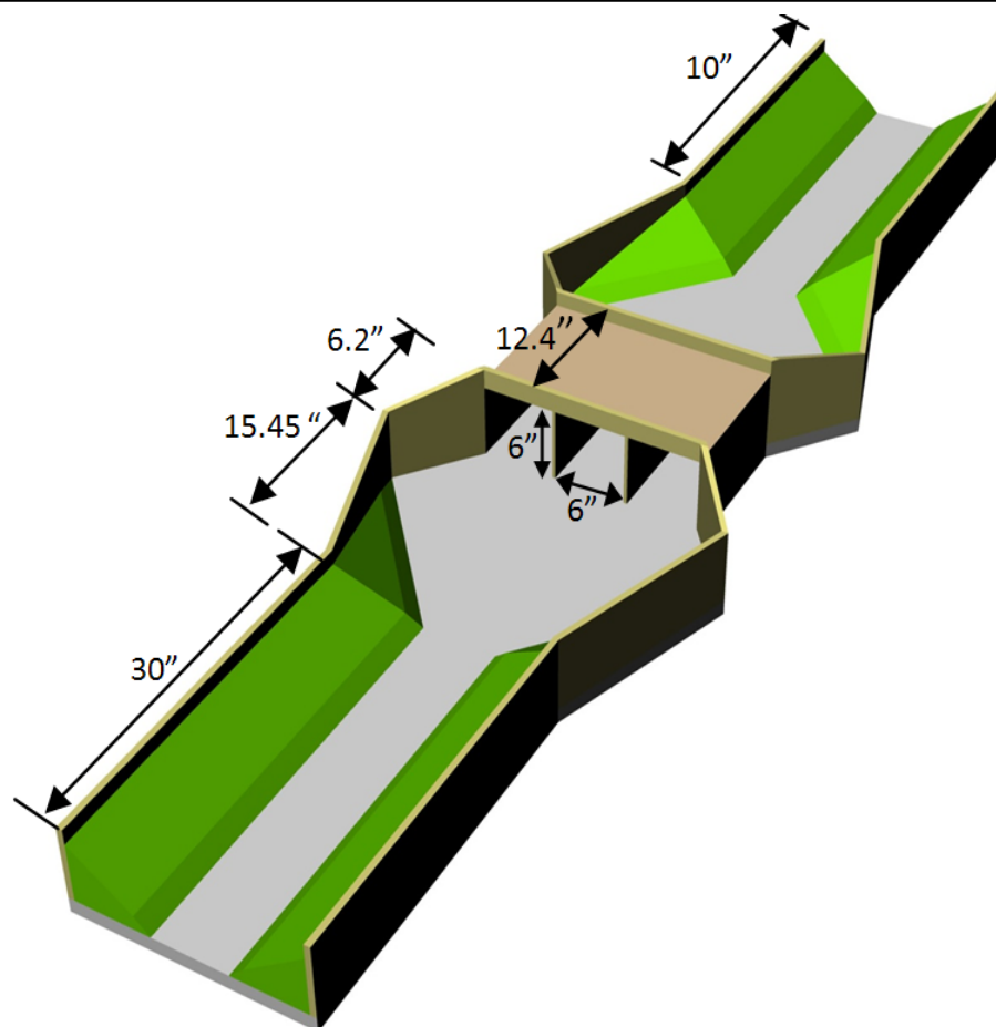
Figure 4-2-10 Layout of the culvert model B
