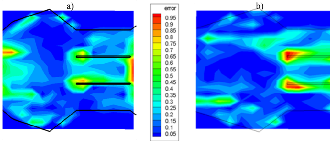
Figure 4-4-8 Comparison of average velocities error between numerical simulations (with FLUENT) and experimental results (with LSPIV) : (a) flow Case B, and (b) flow Case C
