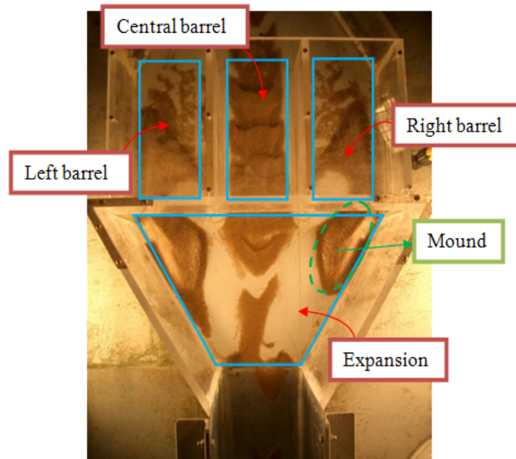
Figure 4-2-6 Sediment load distribution
