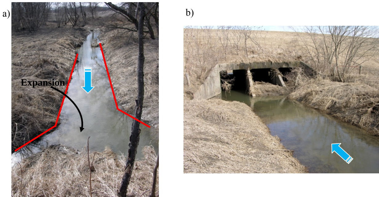
Figure 1-1. Culvert site at Iowa City, blue arrow indicates flow direction: a) upstream view from the culvert, b) downstream view from the channel left bank
