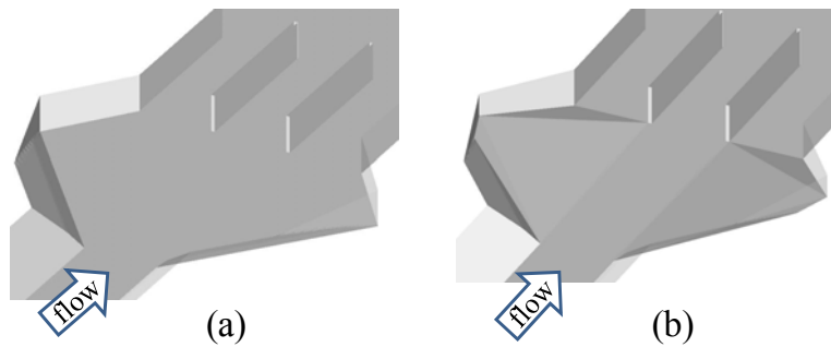
Figure 4-4-1 Calculation domains for numerical simulation: (a) domain for model 1/20B, (b) domain for model 1/20B+FA design
