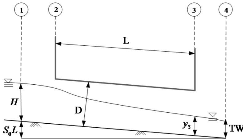
Figure 2-3-7 Culvert with unsubmerged upstream and downstream
