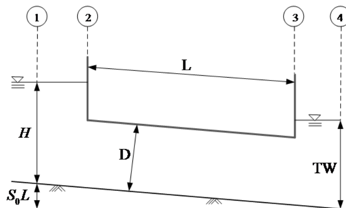
Figure 2-3-6 Culvert with submerged upstream and downstream
