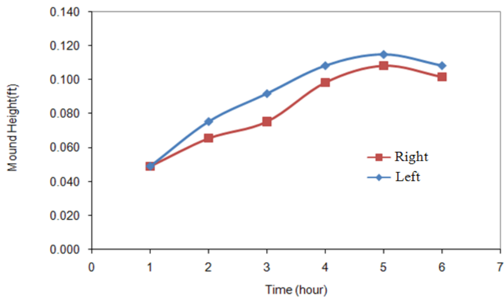
Figure 4-2-9 Dune height variation with time from one-hour to six-hours
