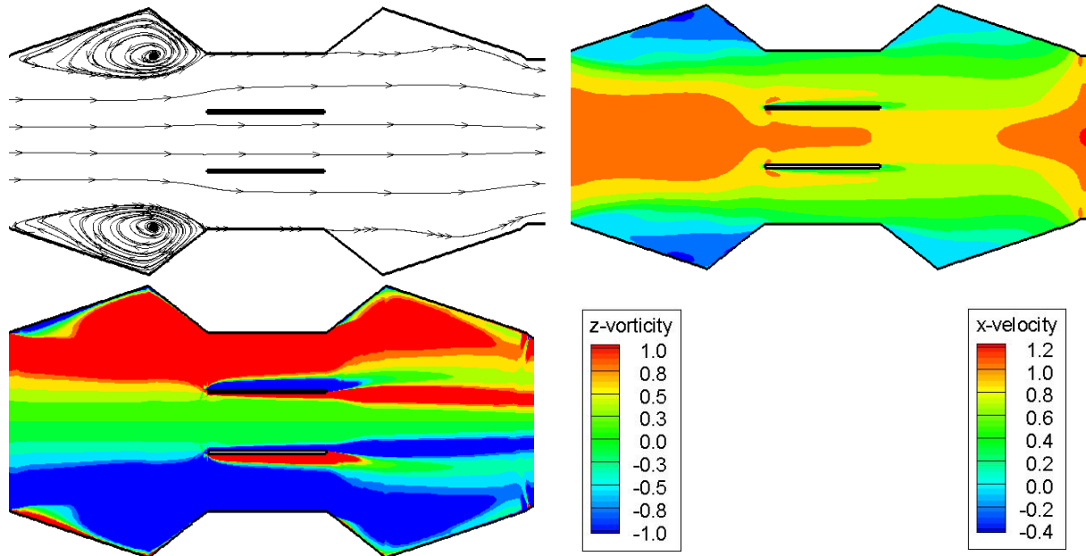
Figure 4-4-5 Near surface flow field for flow case C obtained with numerical simulations: (a) streamlines (b) streamwise velocity (c) out of plane vorticity
